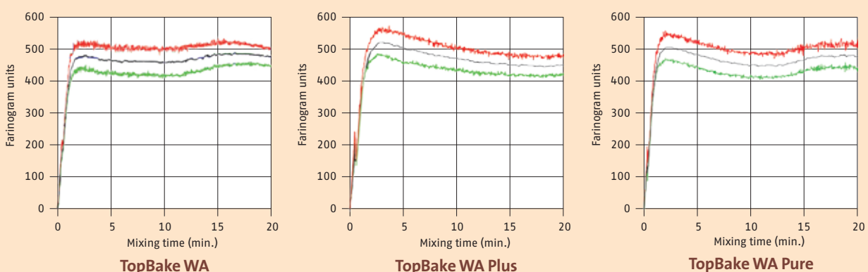
Fig. 1: Farinogram at 1% dosage level (wheat flour, 0.55% ash)
